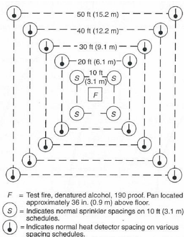
FIGURE A.17.6.3.1.1(c) Fire Test Layout.
